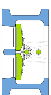
Wafer Type, Dual Plate
